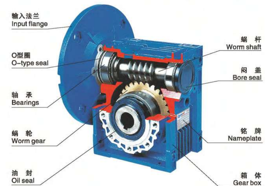
RV 蜗轮减速机 RV Worm-gear speed reducer
