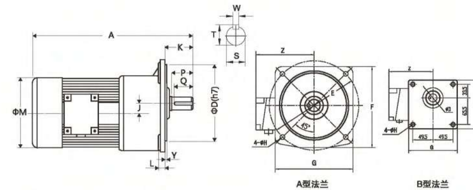
安裝尺寸 (Dimensions)
