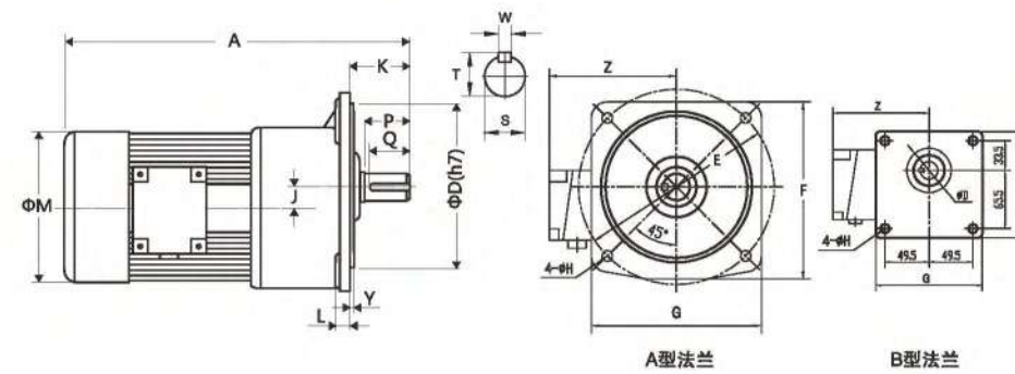
安裝尺寸 (Dimensions)
